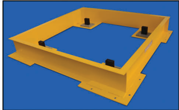
Protective safety yellow framework includes lag down holes and "Nylatron"® Non conductive load cell mounting blocks.
