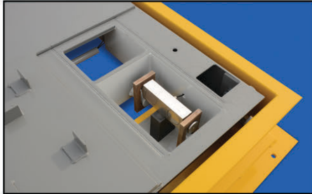
Top access to load cells, polycarbonate NEMA 4x junction box and check stop adjustments.
